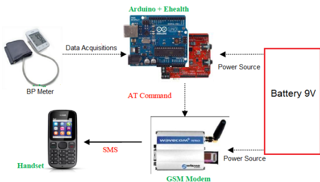
Fig 4. Hardware Implementation
