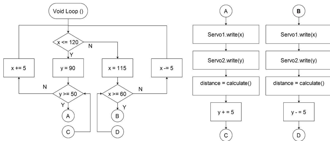
Gambar 5. Flowchart pergerakan motor servo
