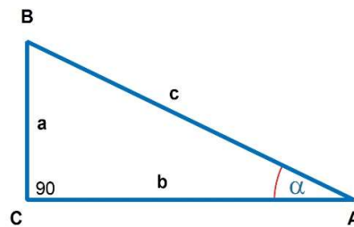
Gambar 3. Trigonometry
